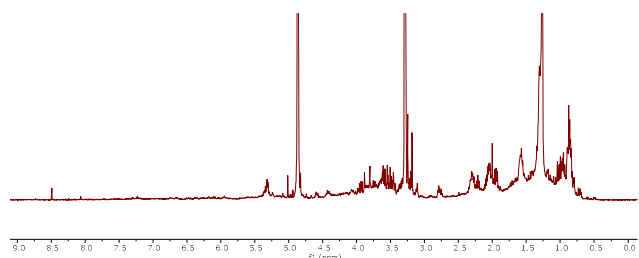
Fig. 6. 1 H-NMR spectrum of crude methanol extract of leaves of C. patulum .
