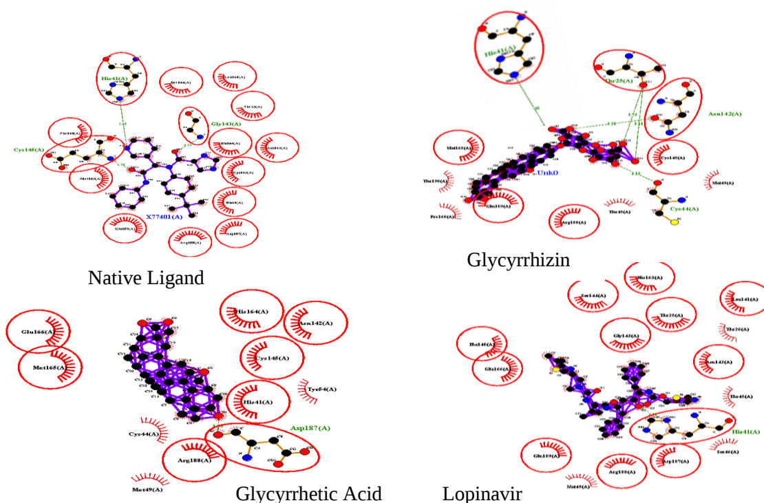
Figure 4. Interaction of ligand amino acid residues and non-structural protein 3 receptors with PDB ID: 6W63 in 2 dimensions
