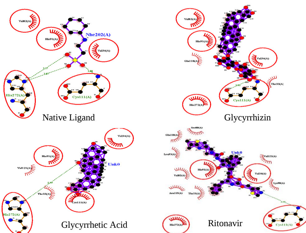
Figure 3. Interaction of ligand amino acid residues and non-structural protein 3 receptors with PDB ID: 6VXS in 2 dimensions
